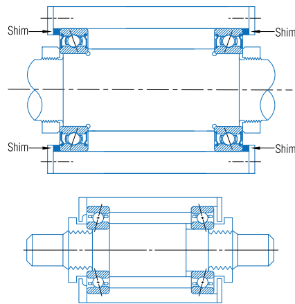
Fig. 7. Axial adjustment.
