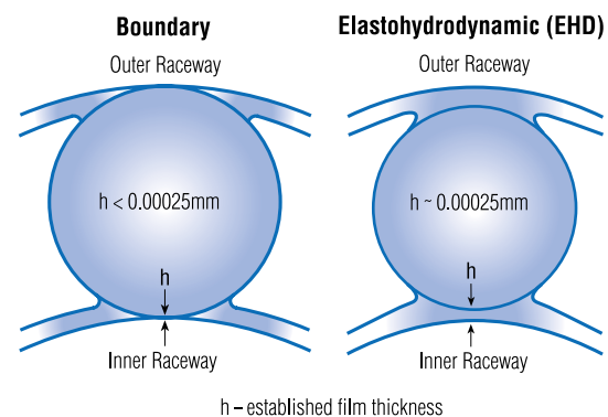
Fig. 13. Lubrication Regimes.
