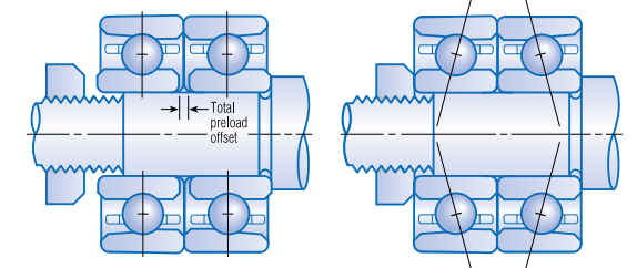
Fig. 8. DB mounting.
