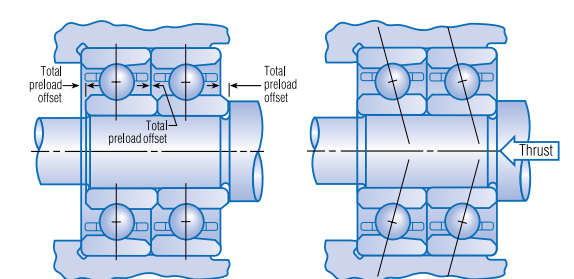
Fig. 10. DT mounting.
