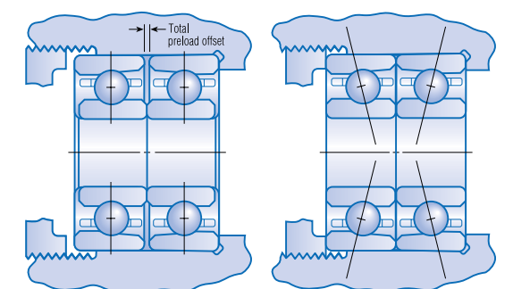
Fig. 9. DF mounting.
