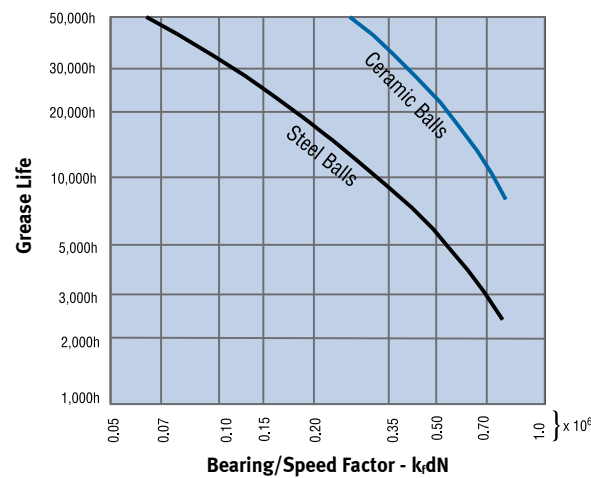
Fig. 20 . Grease life computation for normal temperatures.
