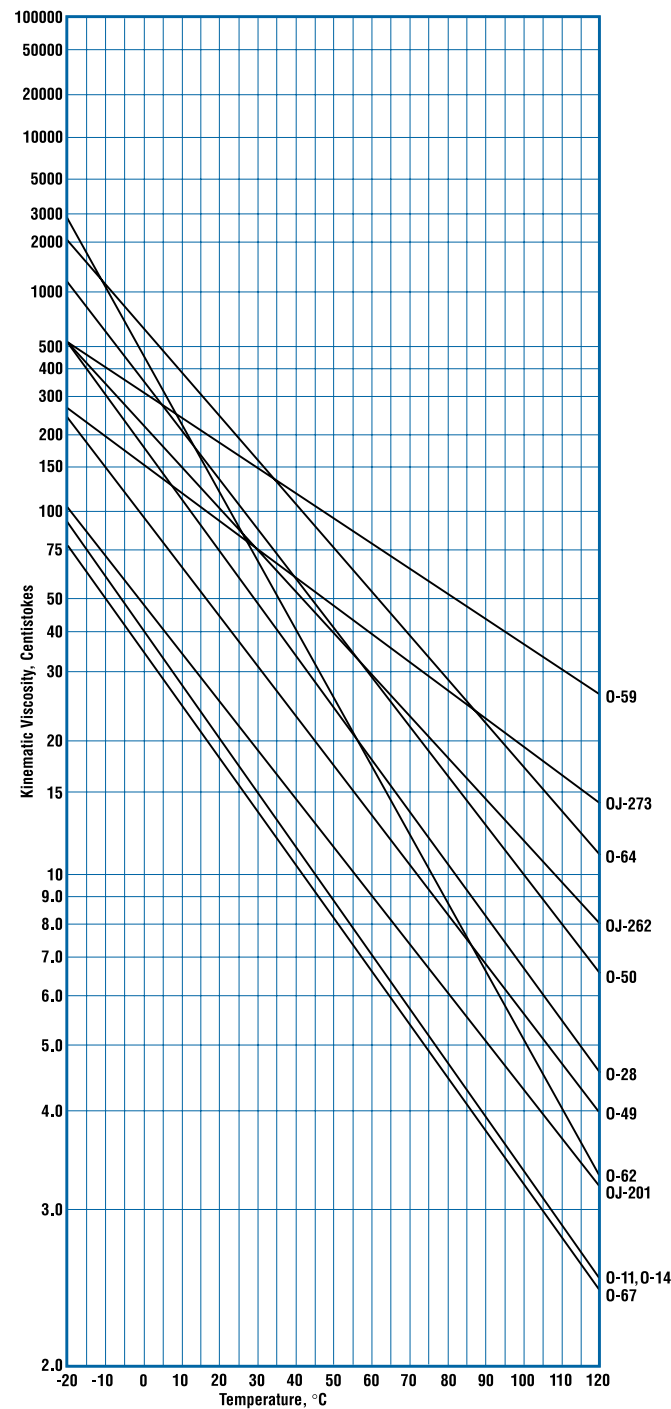
Viscosity graph for several typical oil lubricants.
