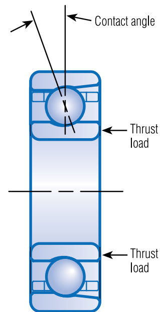
Fig. 4. Contact angle refers to the nominal angle between the ball-to-race contact line and a plane through the ball centres, perpendicular to the bearing axis.
